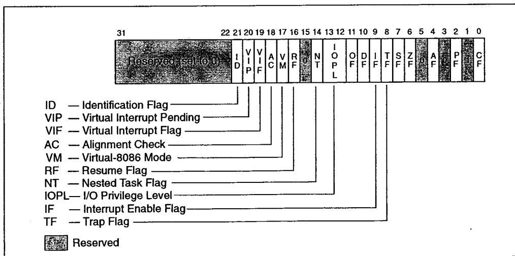
Figure 2-3. System Flags in the EFLAGS Register
