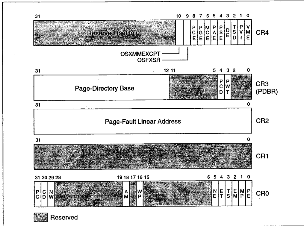
Figure 2-5. Control Registers
